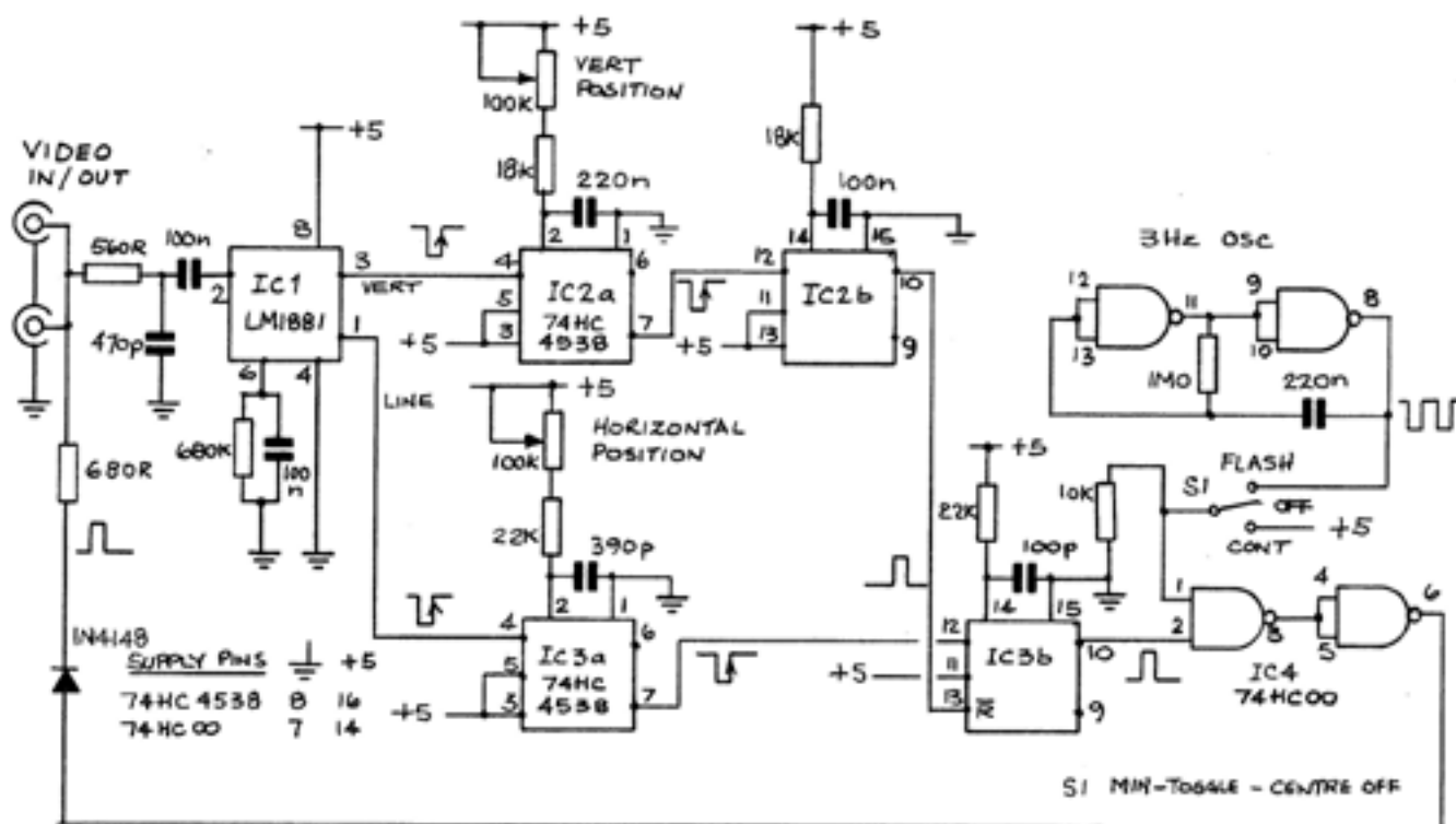
Figure 2 - Circuit Diagram
